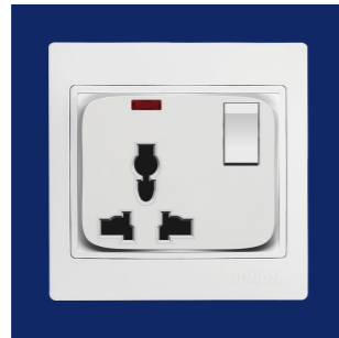
Ref.-no. R811N/9HZ/13 Description 13A 250V~
