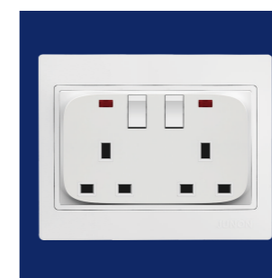
Ref.-no. RF821N2/9H2/13 Description 13A 250V~
